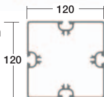
RC120-4 Aluminium profile
